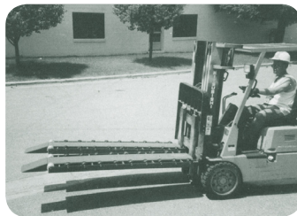
Attaches to forklift and is used to pick up pallets directly from ground. Note the beveled nose plate.
